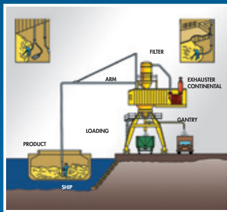
Vacuum conveying
