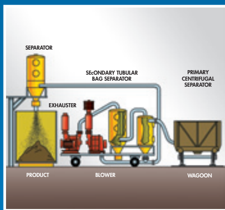
Pneumatic conveying
